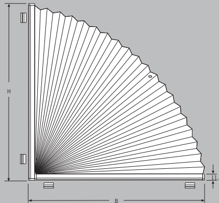
SR 2 fixed width = radius
